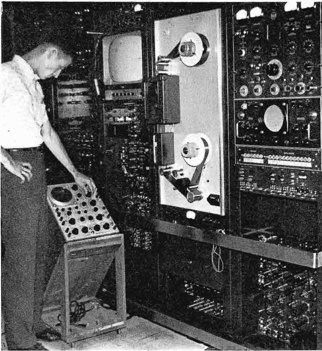
FIG. 11. RCA TRT-1B TV Tape facility in the control room at the downtown studios. WTVM uses this recorder for commercial spots and programs.
