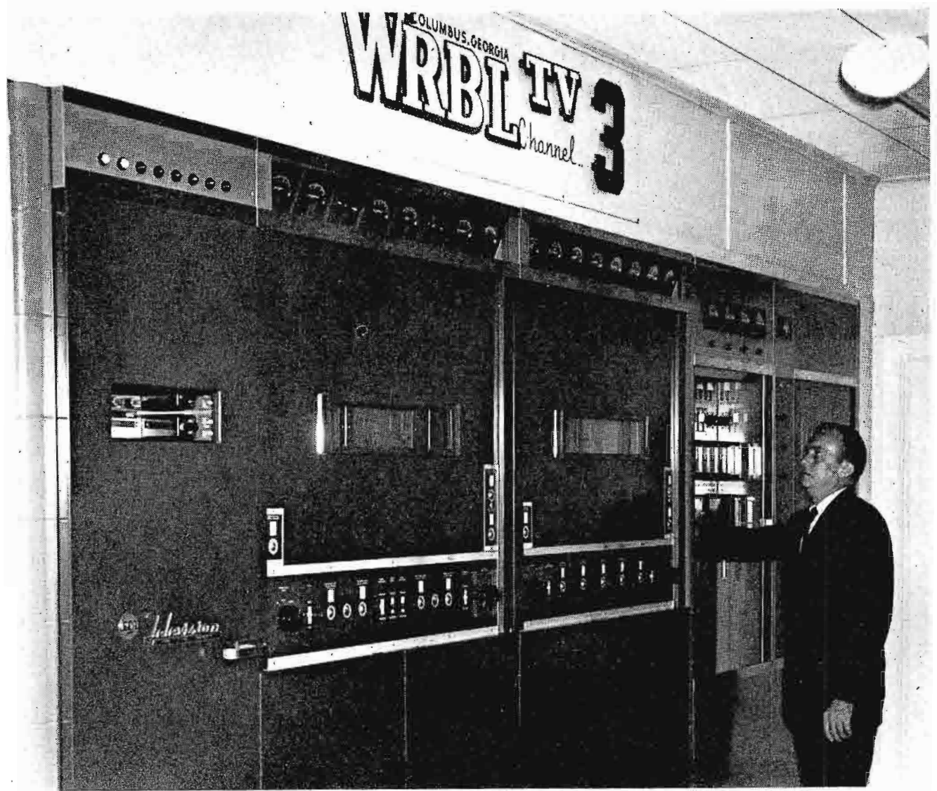
FIG. 8. WRBL-TV employs 25-kw Type TT-25CL TV transmitter.
