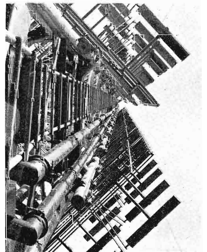
FIG. 4. Looking up the tower between two of the four stacks of super-gain antennas.
