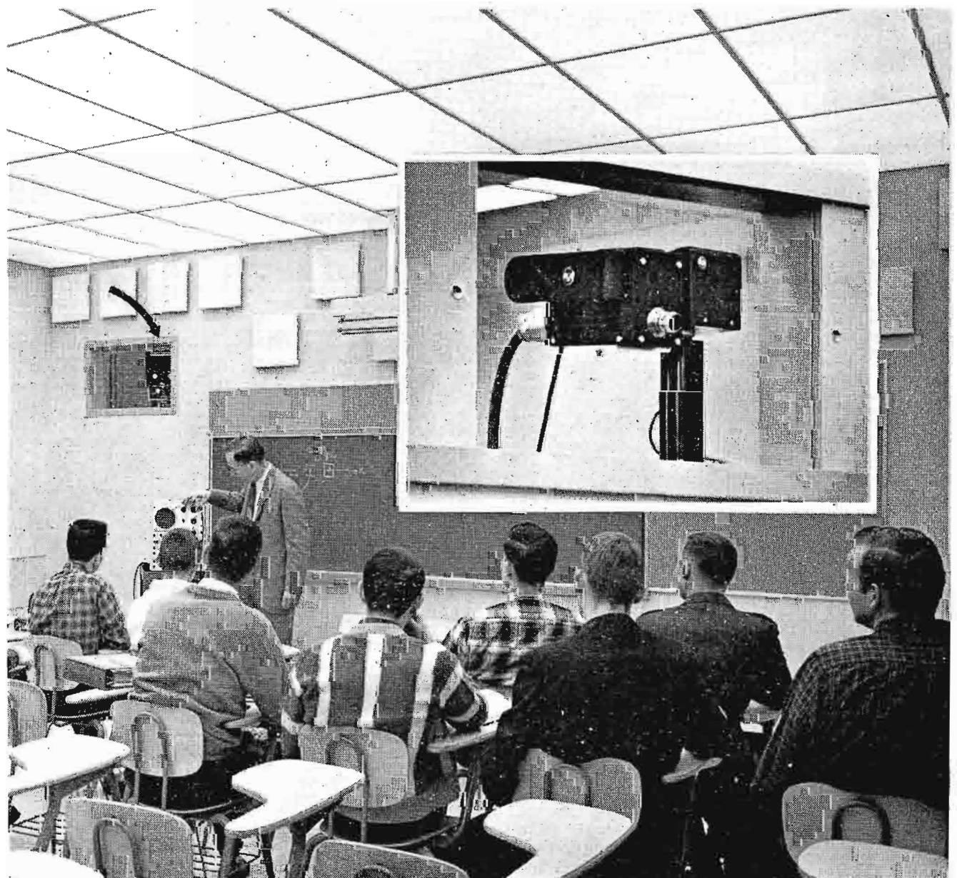
FIG. 15. TV studio-classroom showing TK-15 Camera mounted in front port. Insert shows TK-21 Camera mounted in rear port. There is 375 ft.-candles of illumination in the room.
