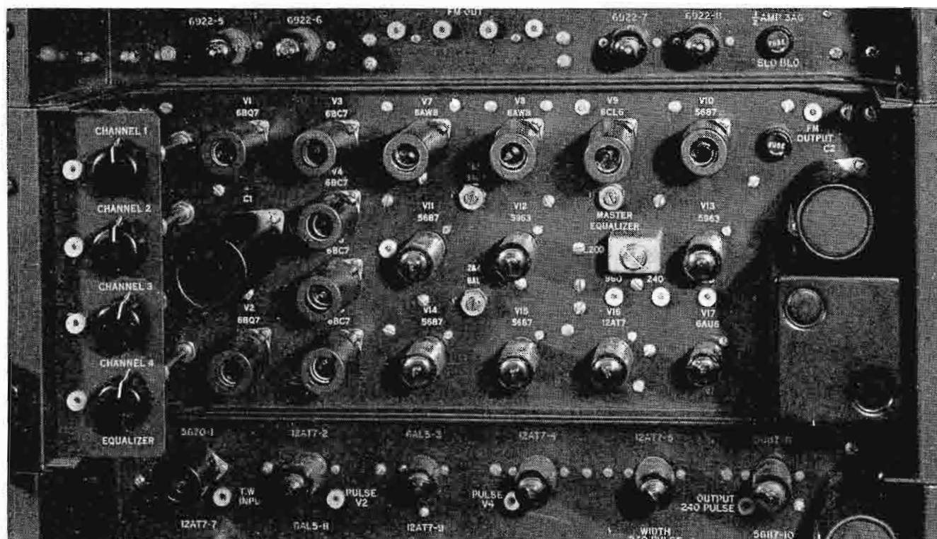
FIG. 4. All FM switching functions are included on a single chassis. A 4 by 2 rf switcher, fully transistorized, has been integrated at the rear of this 2 by 1 switching chassis. A 4-channel equalizer has also been incorporated into this basic unit.
