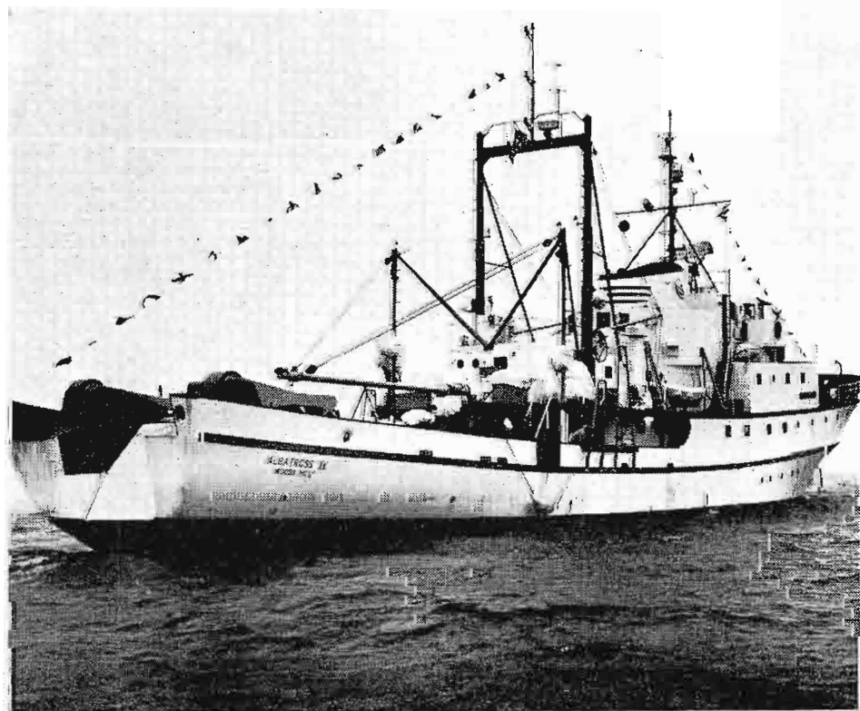
This view of Albatross IV shows two TV cameras in weatherproof housings on crossarms of research vessel's fore and aft masts.
