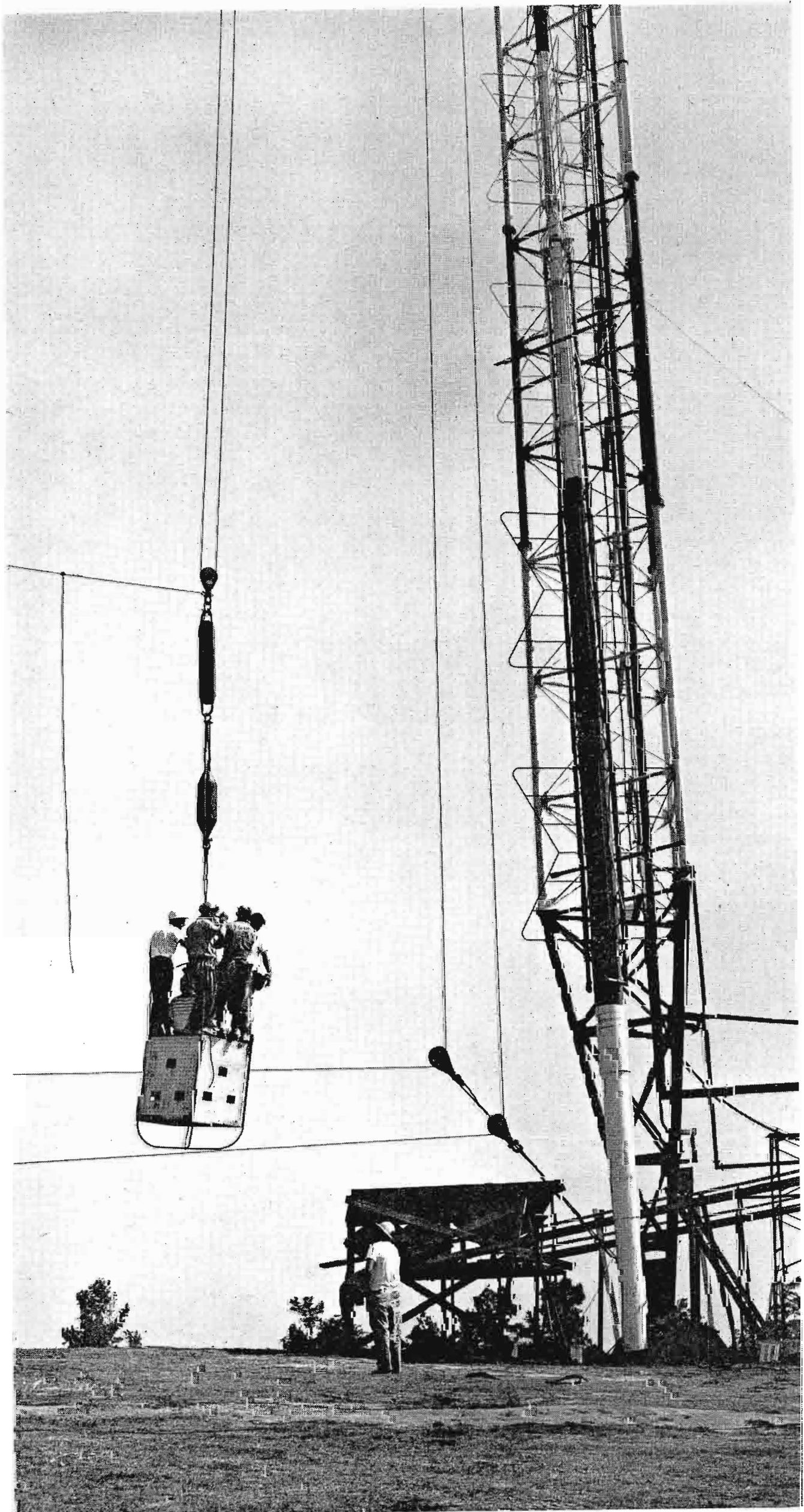
FIG. 5. Riggers used this temporary elevator car (tool basket) to ascend and descend the tower during the extension of tower height.
