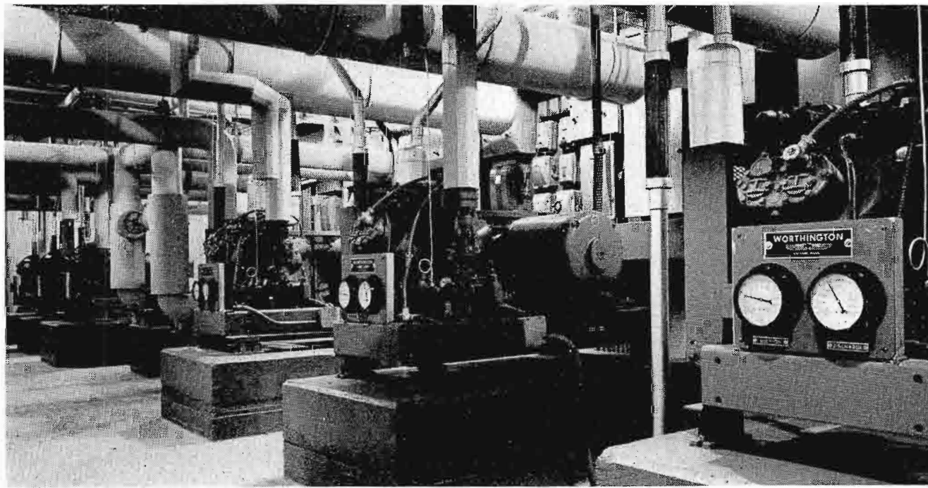
FIG. 29. Compressor-Condenser-Chiller System. Six 30 h.p. compressors are associated with two 800,000 B.T.U. chillers, three compressors to each chiller. System No. 1 feeds treated water at 45 F through a closed circuit to the TV areas of the building. System No. 2 feeds the rest of the building.
