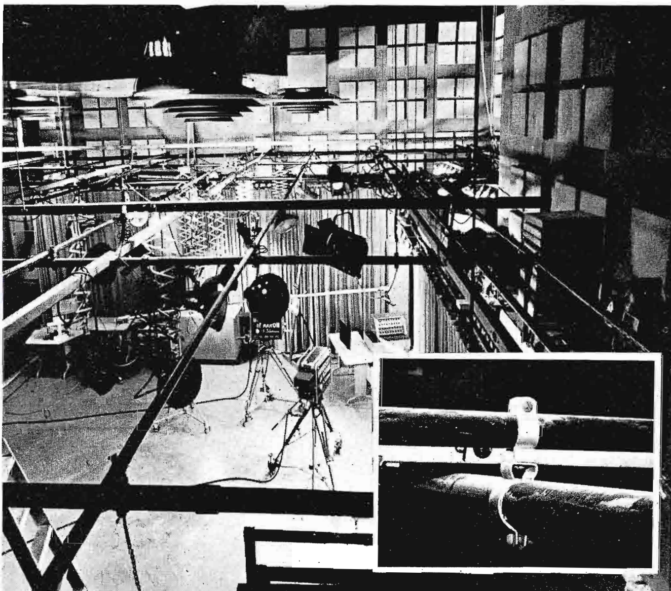
FIG. 5. Studio lighting grid arrangement. (Inset) Detail of special cross pipe clamp.
