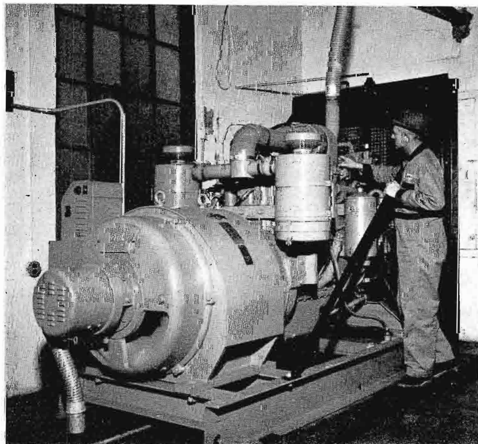
FIG. 10. WRVA diesel electric set rated at 250 KVA. This generator can operate new ampliphase and FM transmitters at full output plus all auxiliary building and lighting equipment. It is entirely automatic in operation.
