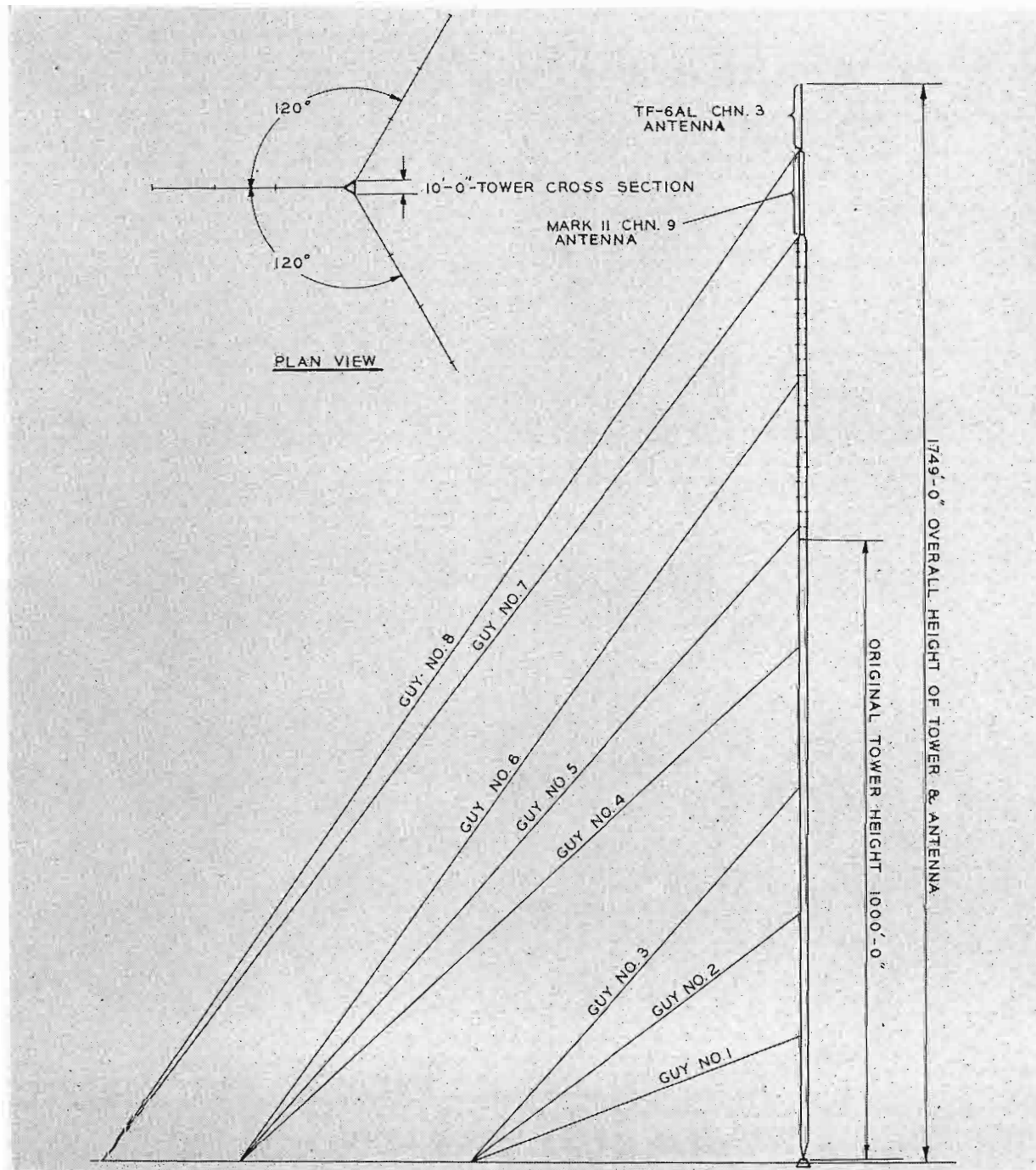
FIG. 7. Side view of tower and antennas showing guy attachments.
