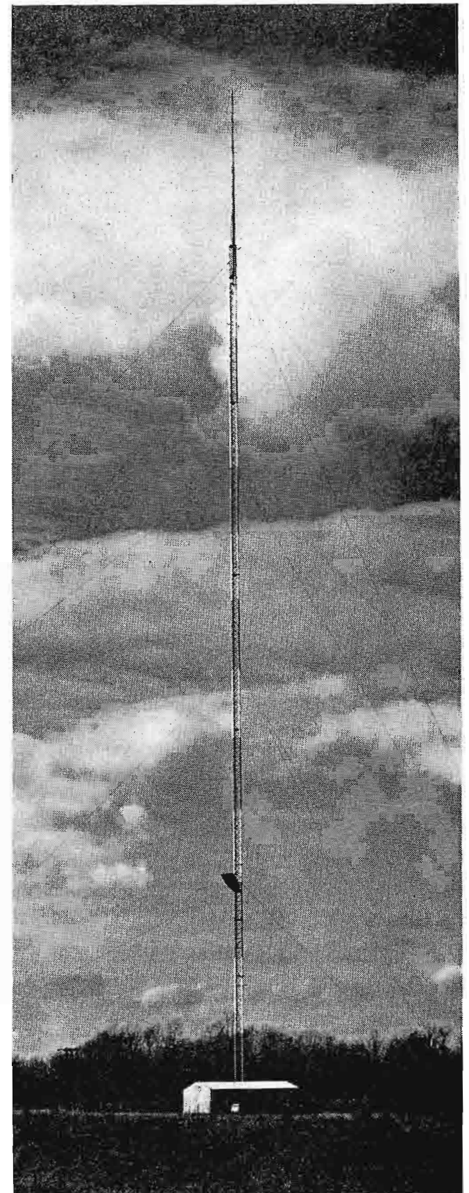
FIG. 33. WAVE-TV transmitter site 500 feet above Louisville. The tower and TF-6AL Antenna overall height are 600 feet. The location, Bald Knob, Indiana, is the highest site in the Louisville area for television towers.
