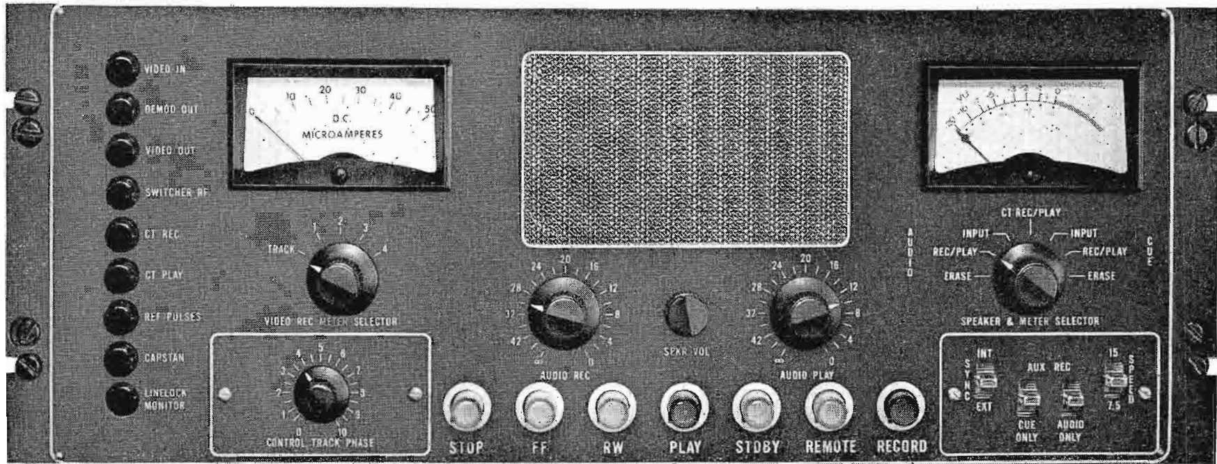
FIG. 2. The functional arrangement of this compact control panel expedites setup, check-out, and operation of the TR-2 Recorder.
