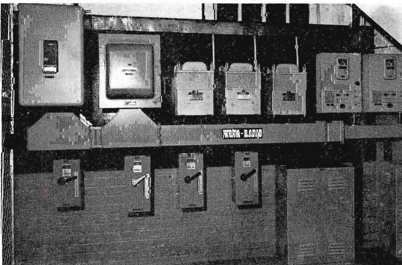
FIG. 3. Immediately below the new RCA 50H, in the basement, is mounted the switch gear associated with the transmitter. To the left of this are the three high voltage transformers enclosed within a heavy wire grating. Mounting this switch gear in the basement has proven entirely practical since the necessity to manually operate these breakers is very rare.
