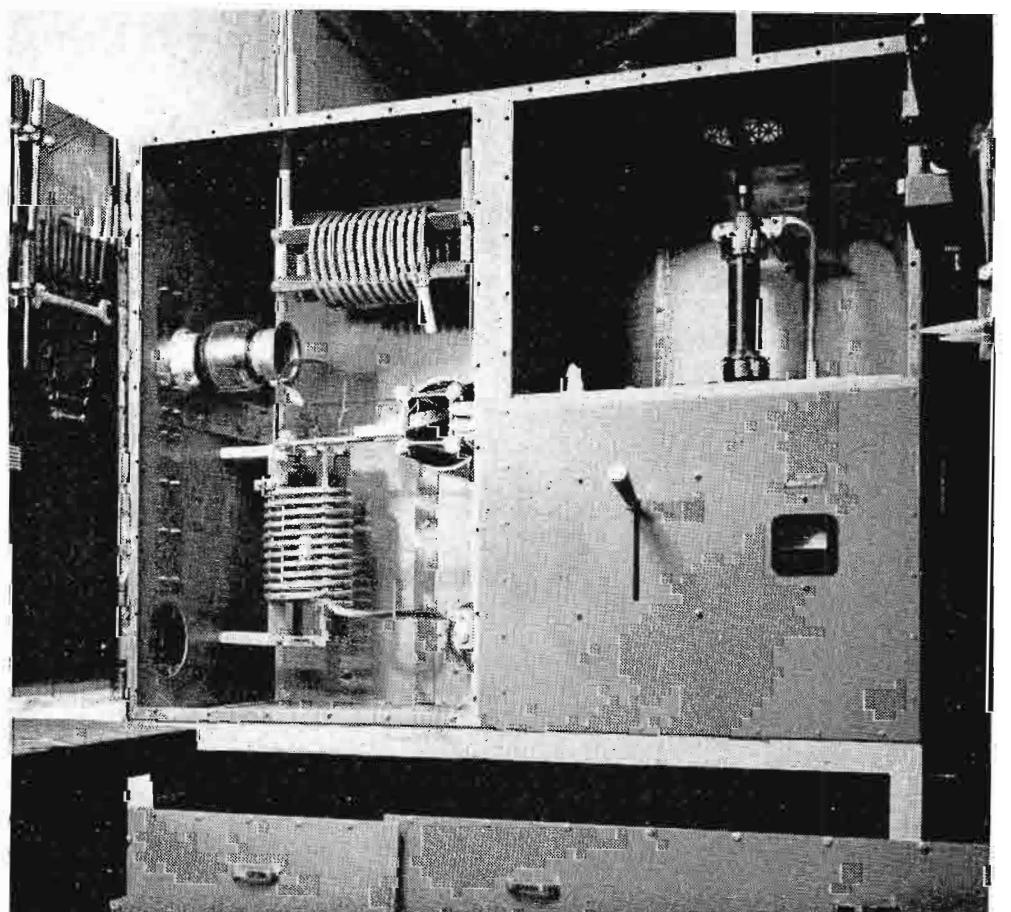
FIG. 11. WRVA 50-kw dummy antenna with covers removed, showing a special matching network on the left with the water-cooled dummy load on the right. This equipment was specifically designed by RCA for WRVA.
