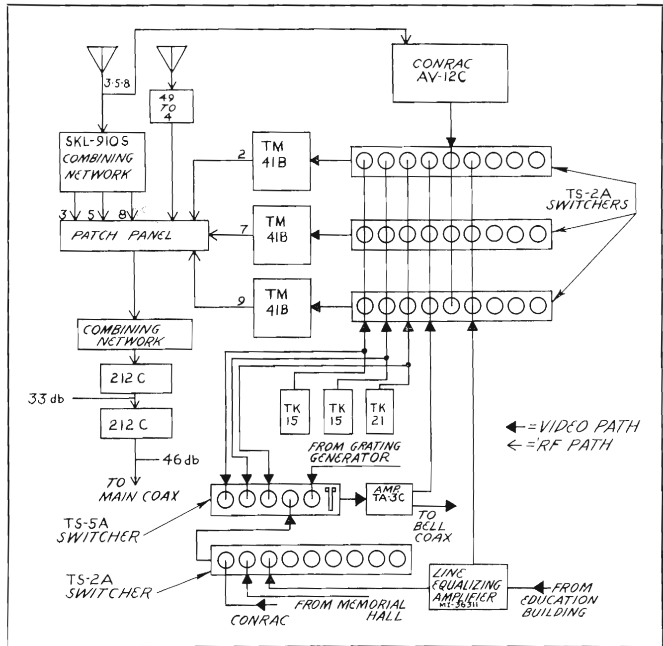
FIG. 10. Interconnection of Video and RF distribution system.
