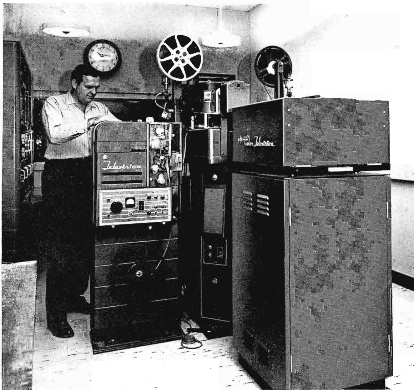
▲ FIG. 19. WAVE-TV film projector room, showing TK-26 3-V Color Film Camera, TP-6 16mm Projector, TP-15 Multiplexer, and random select projector shooting into a periscope. Fred Ray attends the projector.
