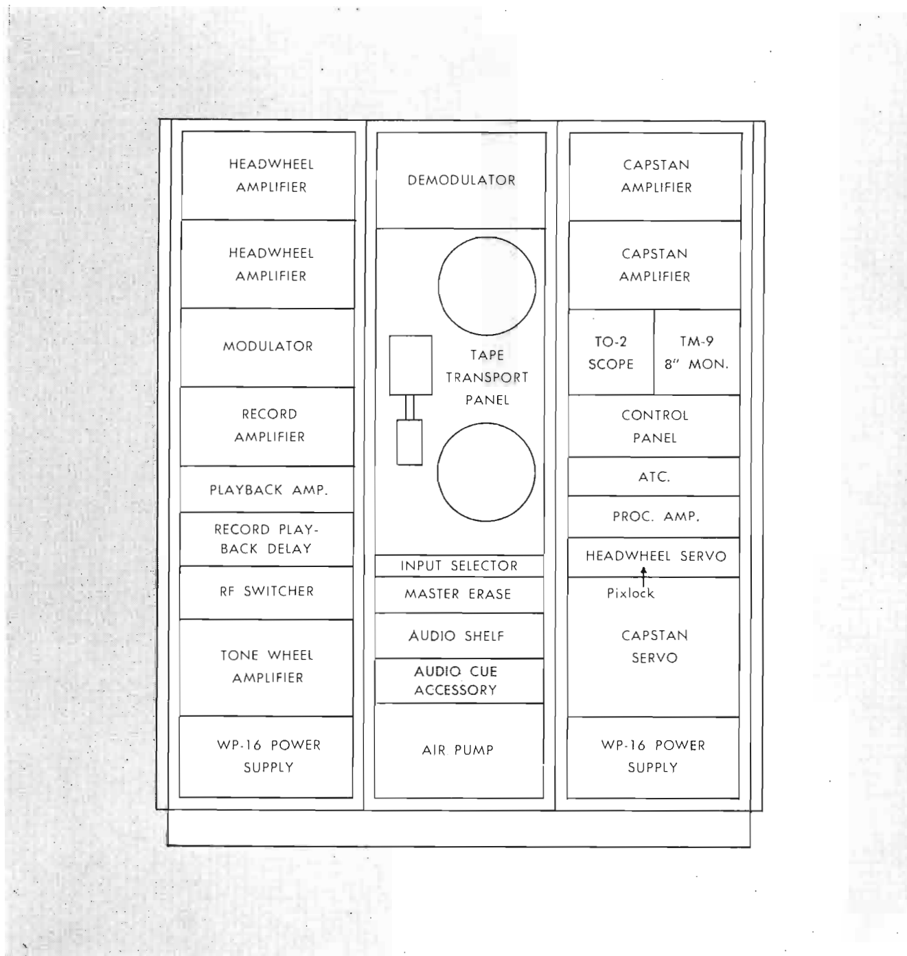
FIG. 6. Functional diagram of the studio model TR-2 Recorder. Mounting space which has been provided for optional accessories is indicated by the gray panels.
