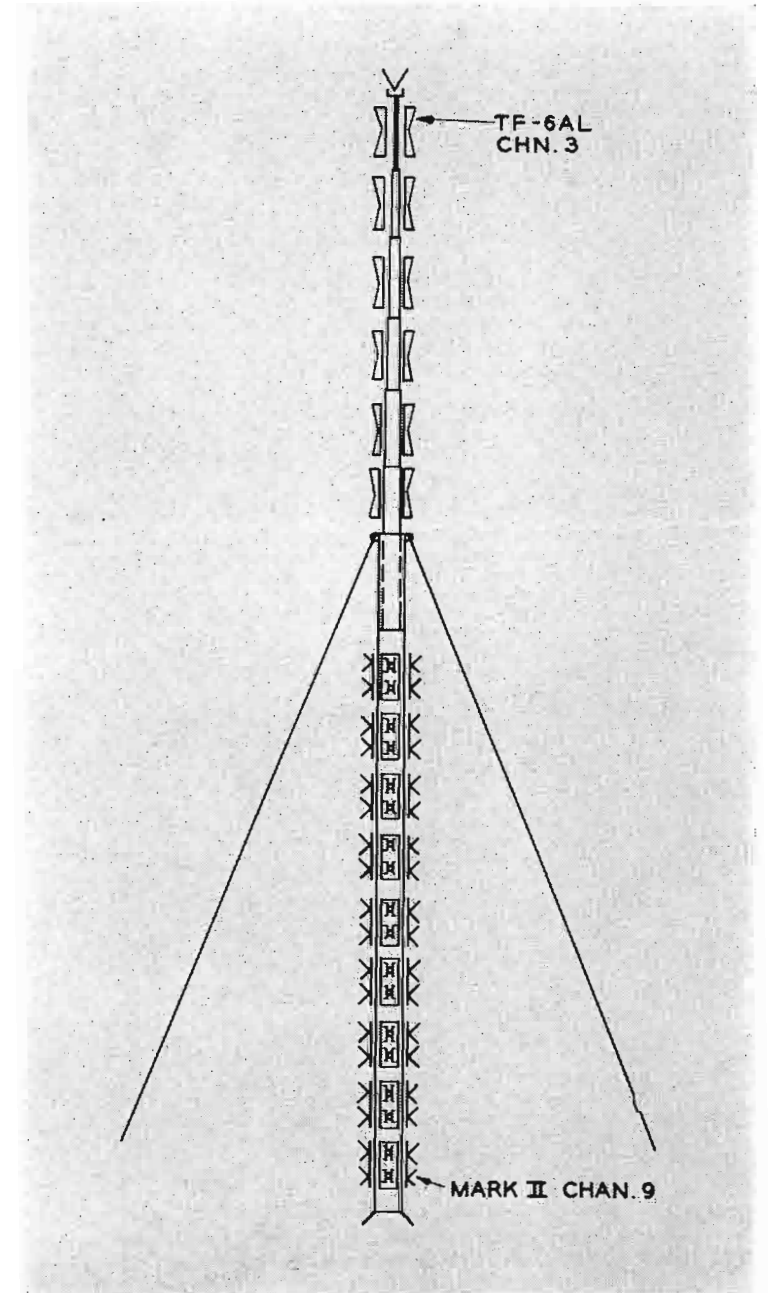
FIG. 8. Draftman's drawing of two antennas "stacked" atop the world's tallest tower.
