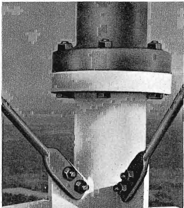
FIG. 10. Tower leg flanges are precision welded for snug fit and ease of erection.
