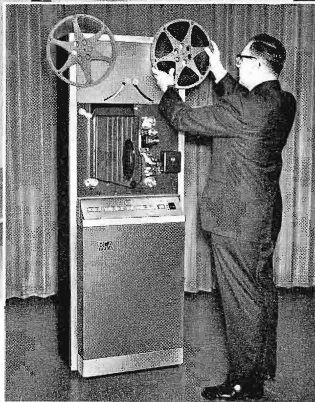
FIG. 11. This display demonstrated transistorized equipment for the modern TV film room. Included were a new vidicon film camera chain, TK-22 (right), and a new 16-mm TV projector, TP-66 (left and inset photo).
