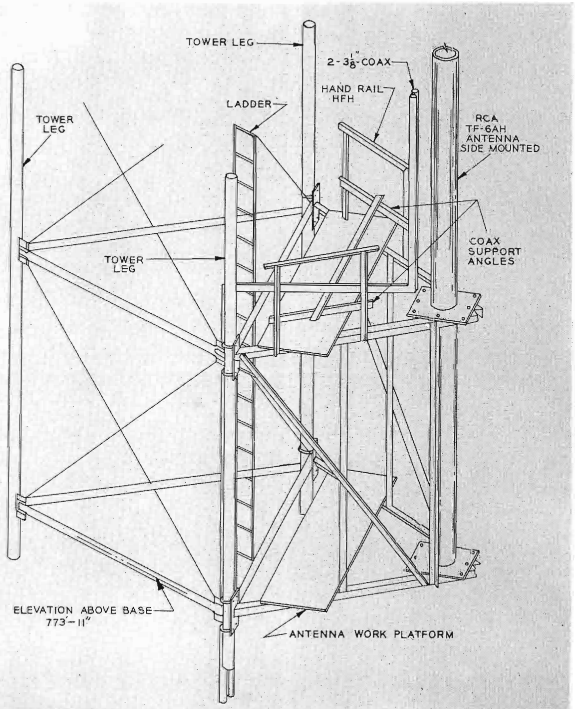
FIG. 11. Side-mounting of temporary channel-9 antenna.
