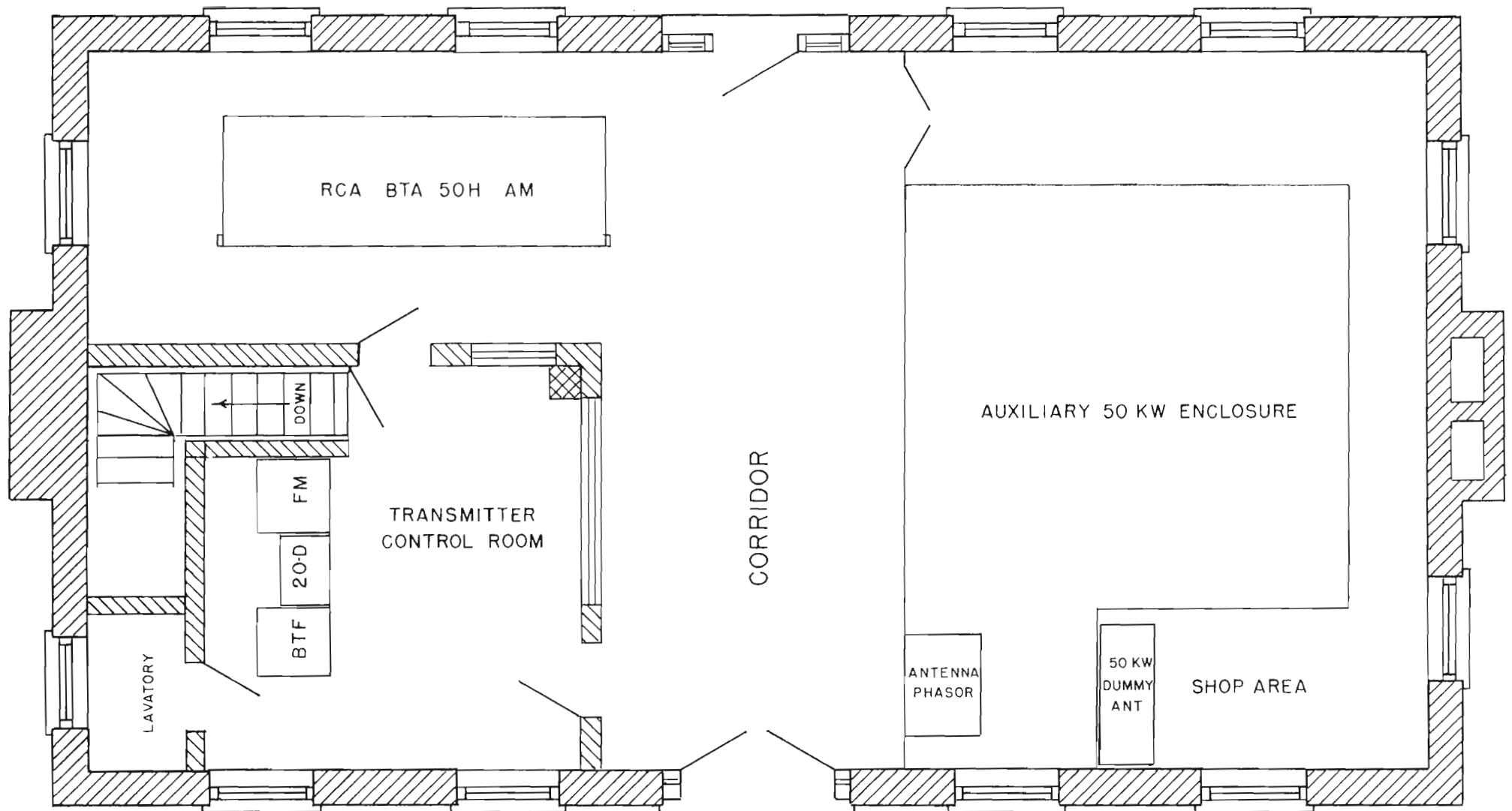
FIG. 5. WRVA-Radio transmitter building floor plan.
