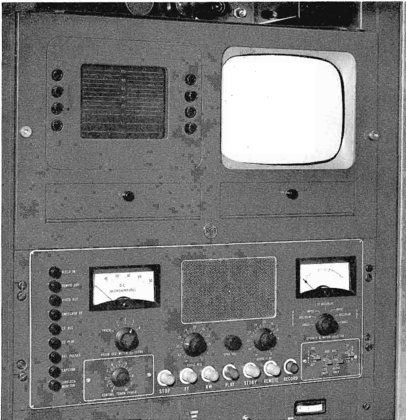
FIG. 8. An 8-inch picture monitor and 5-inch waveform monitor may be mounted immediately above the main control panel. These monitors are especially designed for tv tape recording applications—switching circuits for the monitors are built-in the basic recorder.
