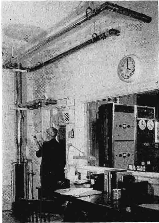
FIG. 7. A problem was solved by bringing harmonic filters of BTF-20D FM Transmitter across control room ceiling and through wall as shown. Line lengths were accurately laid out so both would be equal. The lines lead to wall-mounted diplexer where outputs of two 10-kw amplifiers are combined. Below diplexer is a water-cooled 7.5-kw load, which comes into play in event a 10-kw amplifier needs servicing. This is accomplished automatically and keeps the FM signal on the air without interruption with 50 kw ERP.
