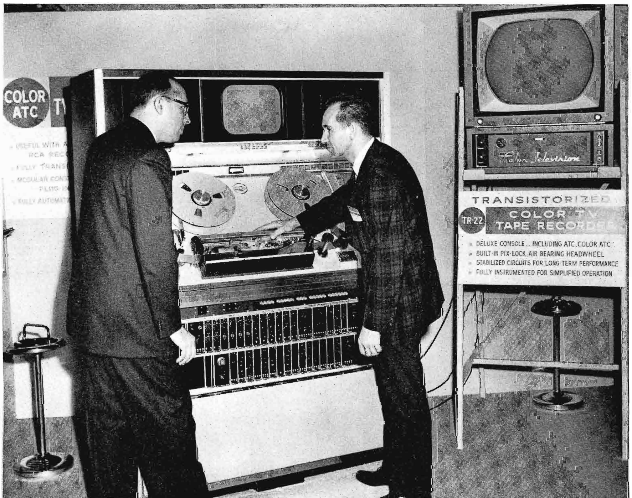
FIG. 4. This deluxe transistorized TV tape recorder, TR-22, was completely outfitted for color taping. New color processing equipment is comprised of six transistorized plug-in modules accommodated in the module bank of the TR-22 recorder.
