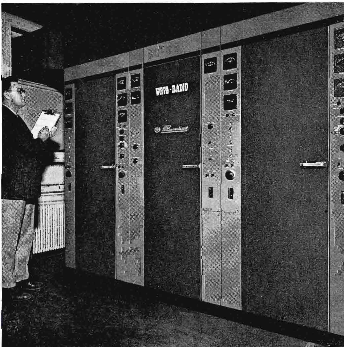
FIG. 6. Transmitter Supervisor, Ted Chezik, at new RCA 20D FM transmitter. Above the 20D, note exhaust duct. This is equipped with booster fans as a safety factor under extremely hot weather conditions. With this arrangement, this excellent FM transmitter is a very cool running piece of equipment.
