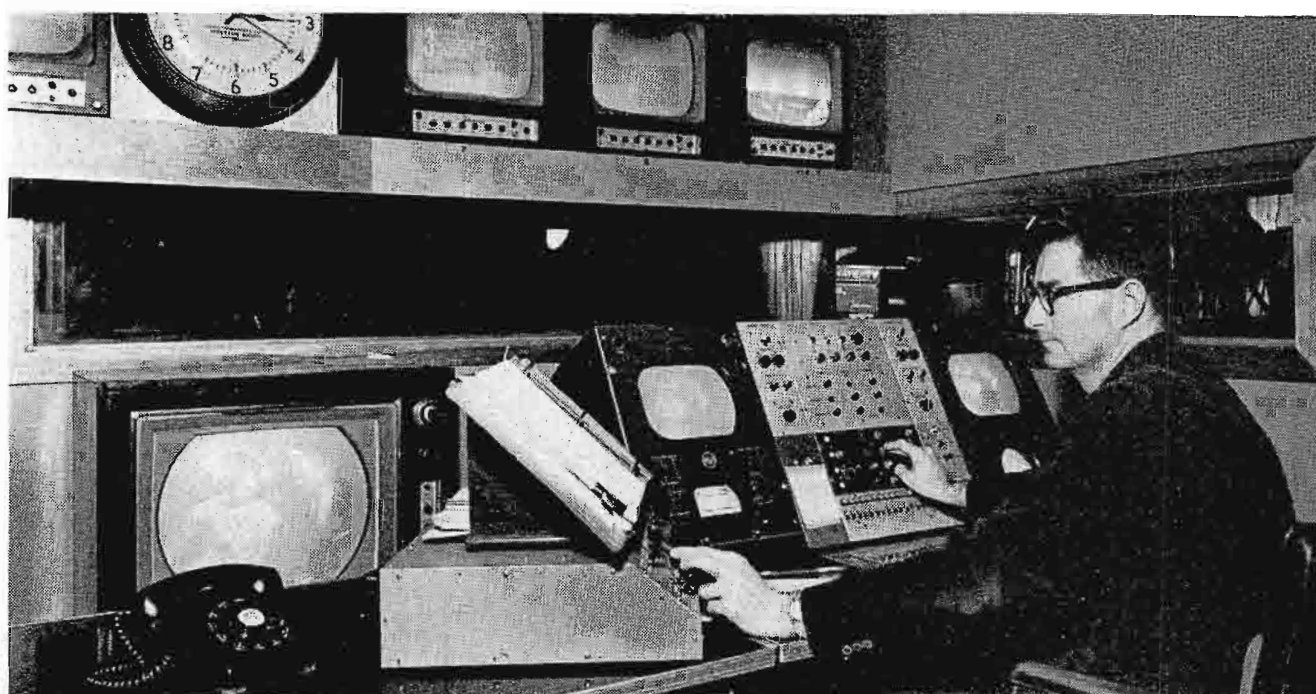
FIG. 22. WAVE-TV control booth, Robert Russell at video switcher. Panel between two TM-6 monitors contains controls for film and slide projectors. Other controls include genlock, network level, stab-amp, and video switcher outputs. Camera monitors are on overhead shelf. Narrow window allows vision into both studios 1 and 2 for director.
