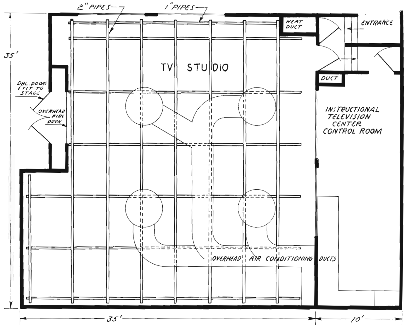
FIG. 4. Instructional television center floor plan. The stage doors open to the University of Akron's Theatre from which CCTV presentations are also originated. The overhead pipes form a grid for supporting studio lighting fixtures (see Fig. 5 below).
