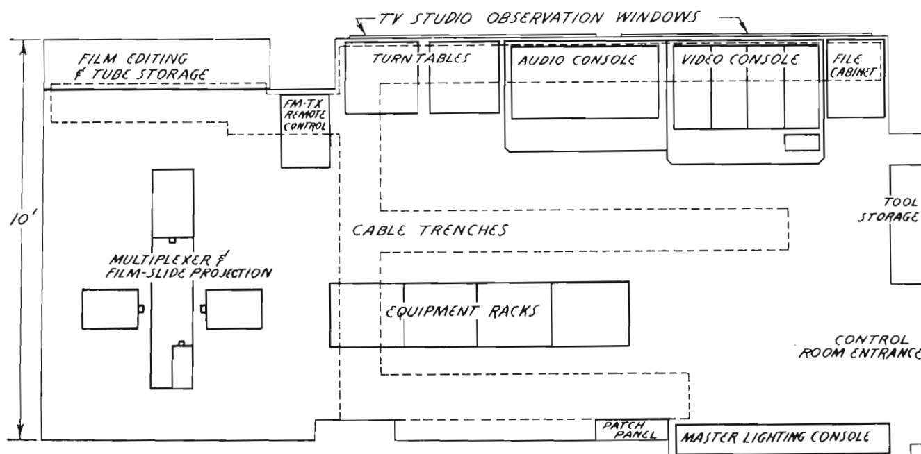
FIG. 6. TV control room layout.
