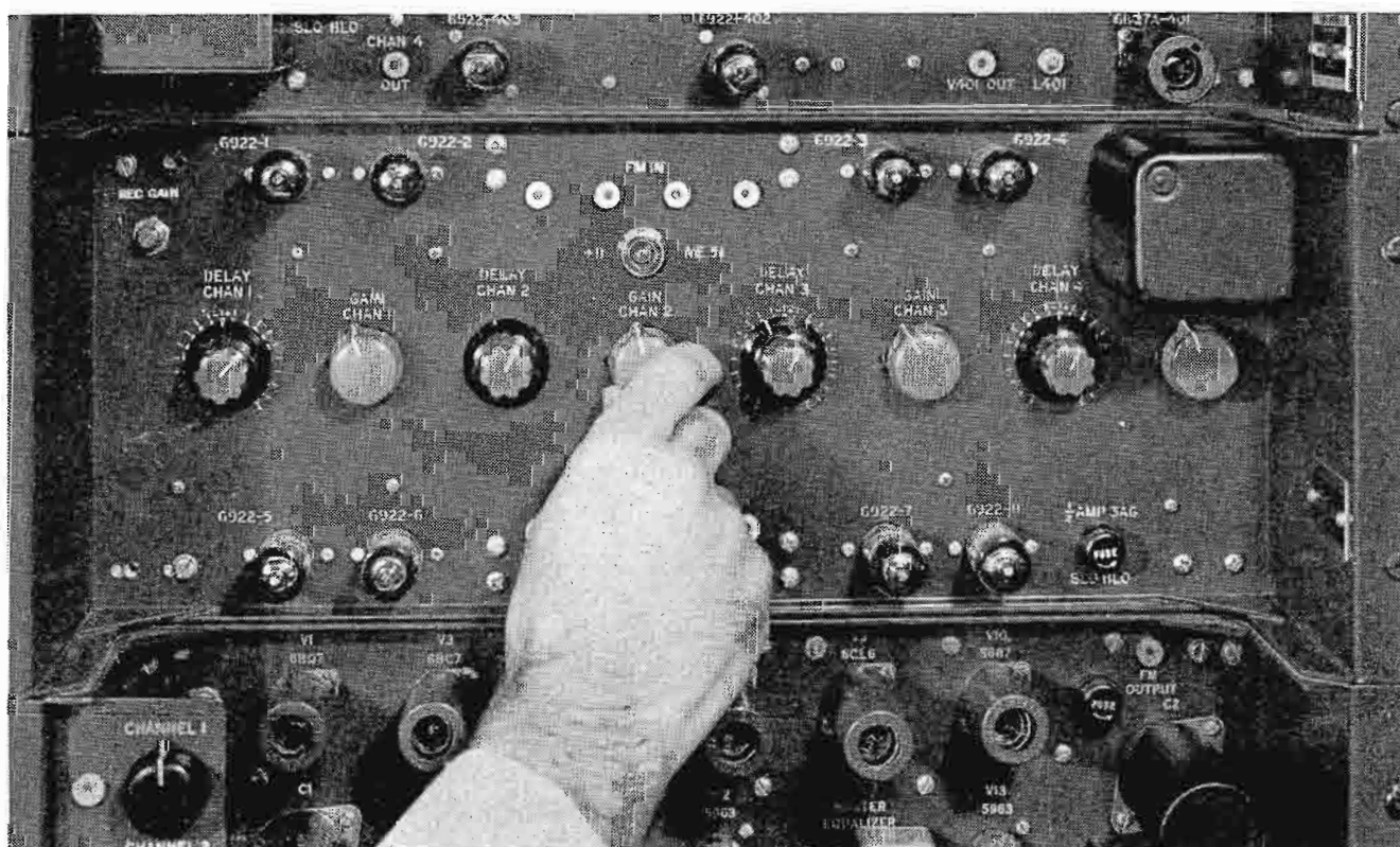
FIG. 5. The electronic quadrature chassis incorporates improved delay lines and dual controls for both recording and playback.
