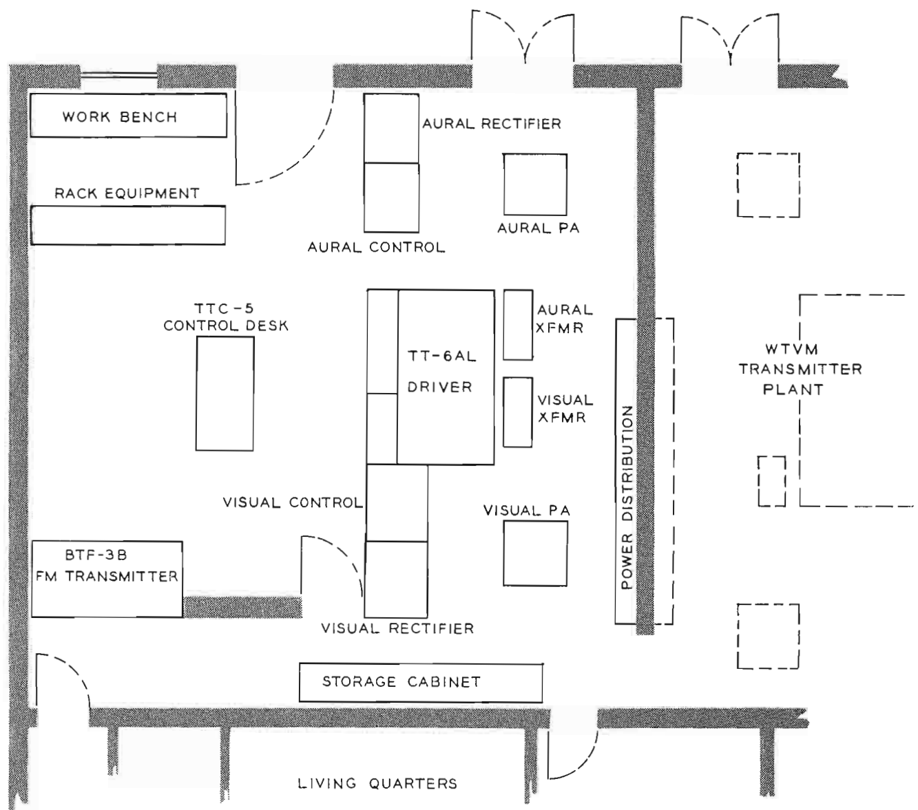
FIG. 9. WRBL's transmitter plant floor plan. The station shares the building as well as the tower. Transmitter personnel live in the "front" part of the building.
