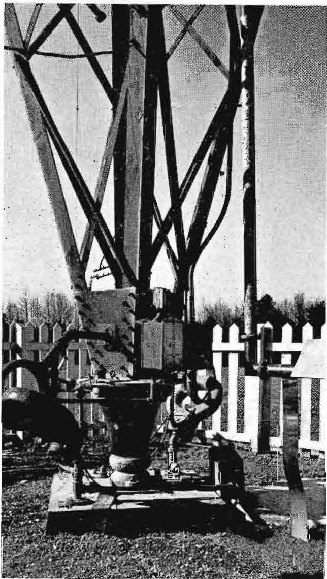
FIG. 12. The FM transmission line drops out of AM tower and tied into ground system. The bottom quarter-wave section of line is suspended by specially designed hangers insulating this section from AM tower. Tuning of stub is accomplished by adjusting movable strap connecting transmission line to tower at quarter-wave point. The horizontal portion of the line runs out a distance of forty feet then enters the ground. From this point to transmitter building line is buried well below frost line. The AM lines are also buried in this manner. The shield over the line protects it from falling ice. Two Austin transformers are shown. One supplies current for heating elements of BFA 12-section antenna. Heaters turn on automatically at low heat when temperature at ground level reaches a low of 40F.
