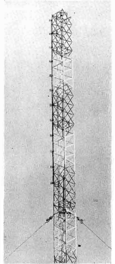
FIG. 9. The RCA BFA-12A center-fed antenna is corner mounted on one of 445-foot AM towers. At the bottom of the FM antenna the transmission line can be seen as it swings into the tower. From this point the line is supported at the cross bracing that carries the ladder, making the line readily accessible for inspection.
