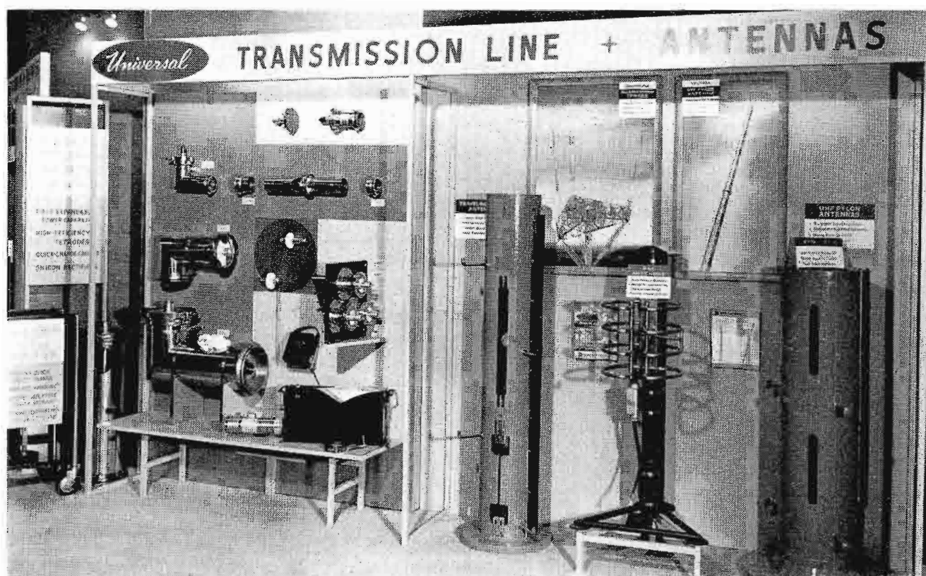
FIG. 9. Transmission line and antennas. The three elbows on the display panel (left) indicate the relative sizes of the 3-, 6-, and 9-inch Universal transmission line. The traveling wave-antenna section appears in the center of the picture with the BFA FM antenna section immediately to the right. A section of the UHF-Pylon antenna stands at the far right.
