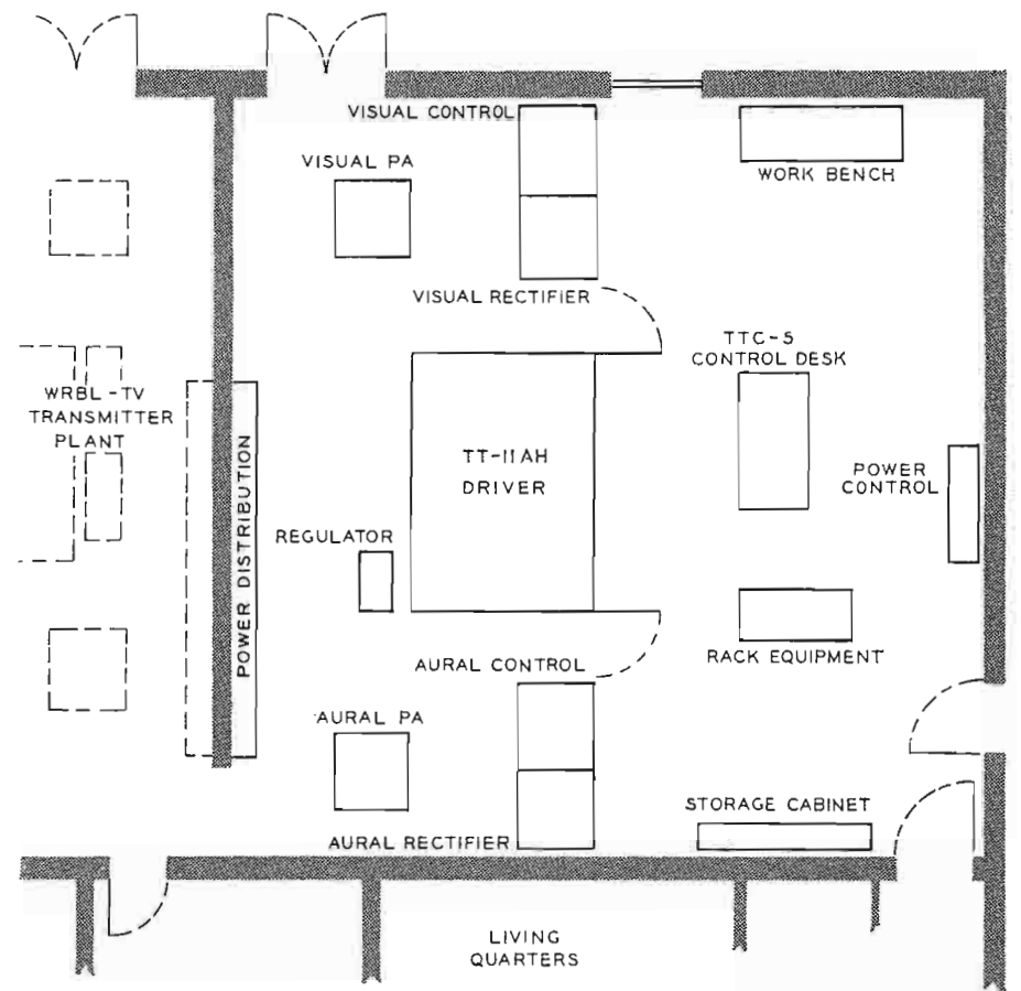
FIG. 10. WTVM shares the transmitter building with WRBL-TV. This floor plan illustrates the roomy, well laid-out plant.
