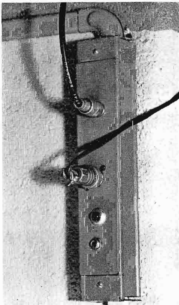
FIG. 13. Classroom TV control stations showing RF and receiver muting cables, talk-back push-buttons, and technician phone jacks. (Left) Surface mounted. (Below) Flush mounted.
