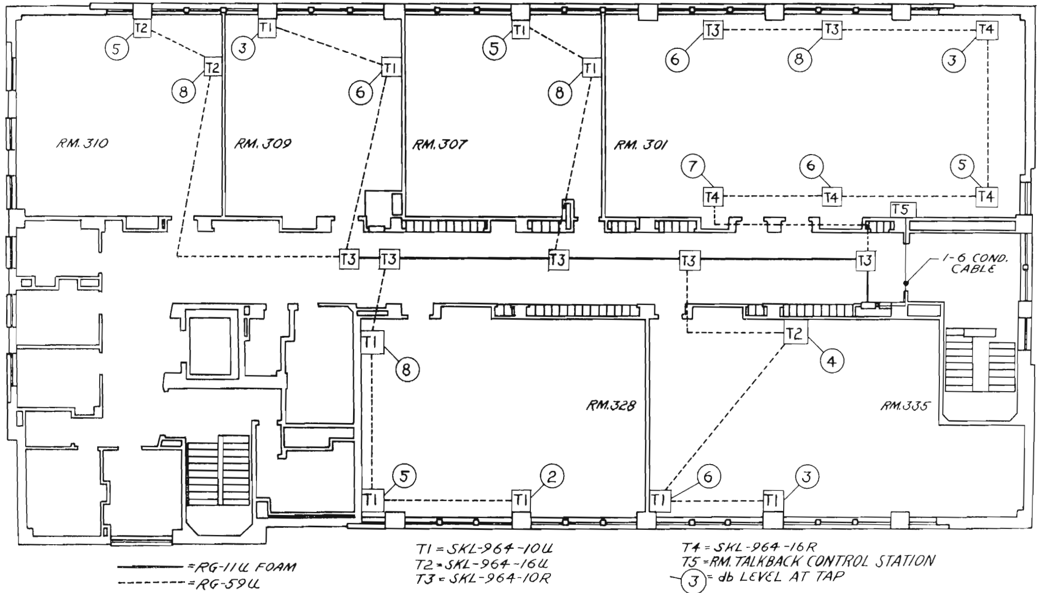
FIG. 9. Third floor plan of University of Akron's College of Education Building showing cable distribution.
