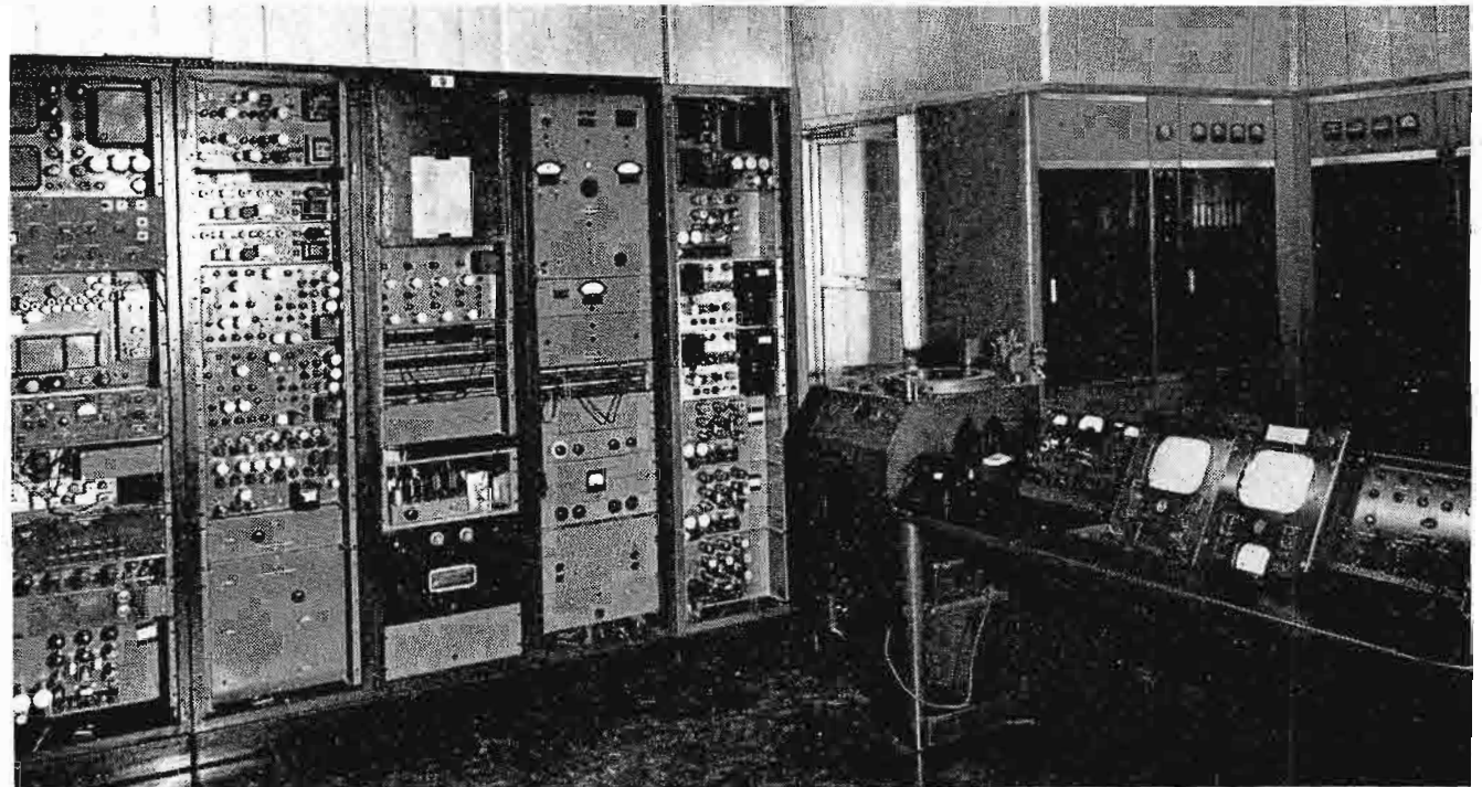
FIG. 35. WAVE-TV transmitter room, showing the control desk and racks of input and monitoring equipment.
