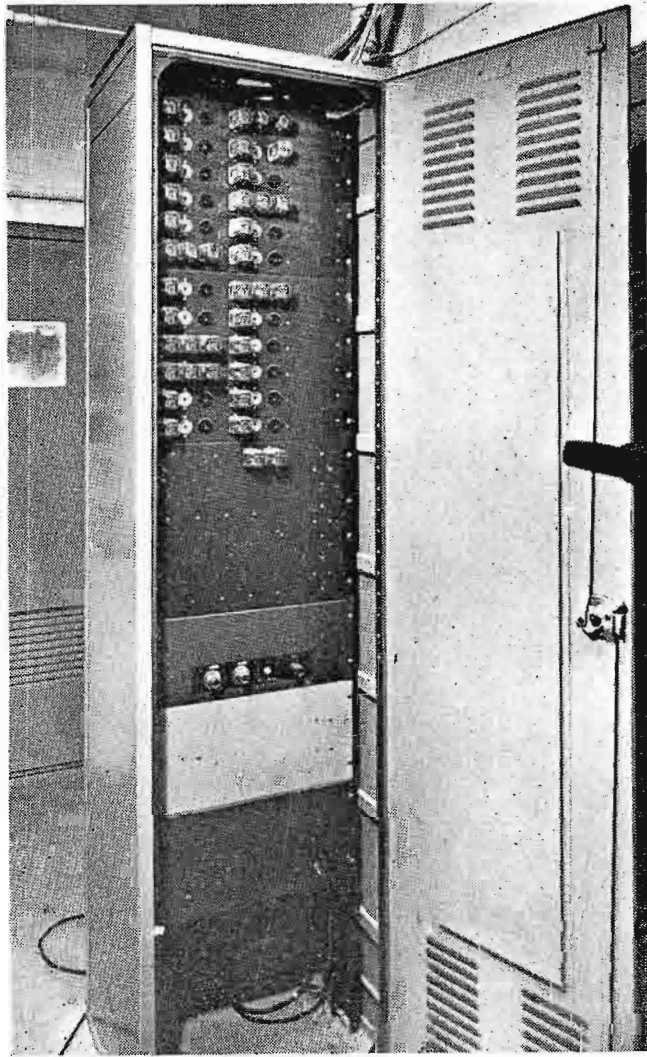
FIG. 14. College of Education talk-back control rack. Contains audio line amplifier, RF amplifier, relays and associated circuitry.
