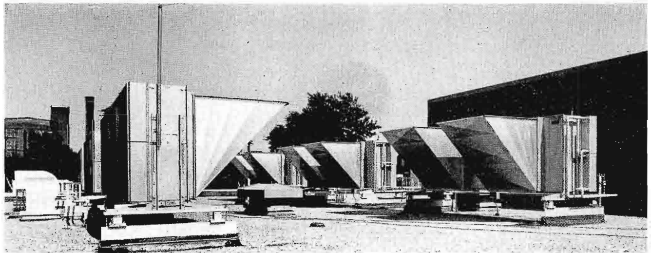
FIG. 30. Each compressor has its individual air-cooled condenser on the roof. No cooling tower is used. Each condenser has two 48-inch fans, belt-driven by one 3 h.p. motor. This system eliminates the problems of corrosion, algae control, water and sewer-tax costs, freeze-up protection.
